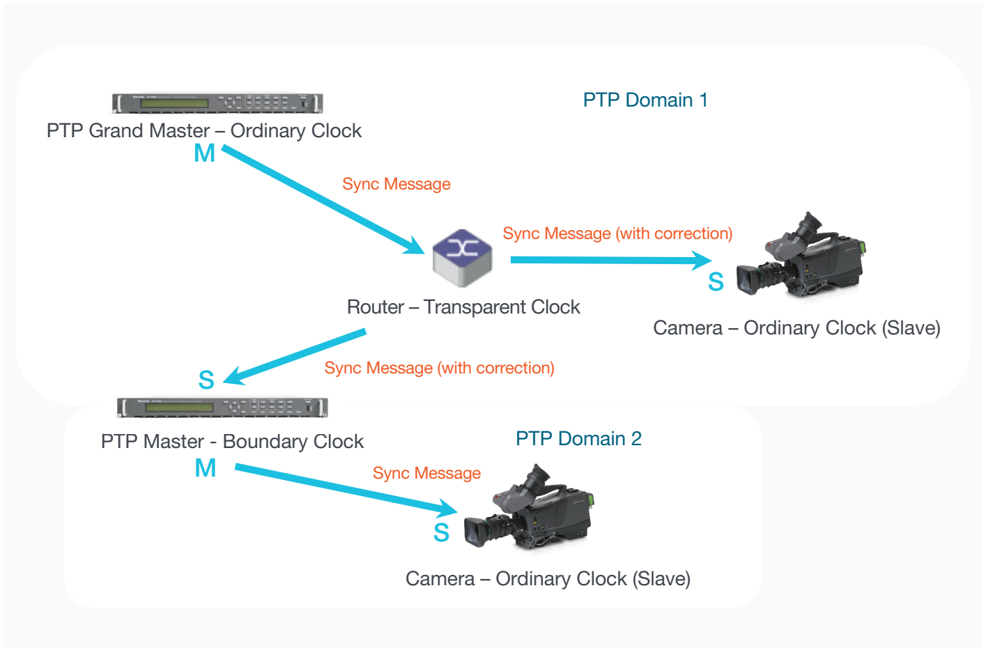
FIGURE 13. PTP Clock Types in a Network.
