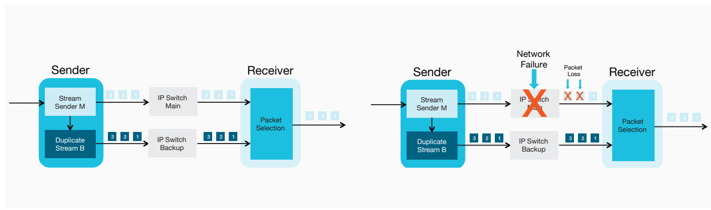
FIGURE 4. SMPTE ST 2022-7 Seamless IP Protection Switching.
