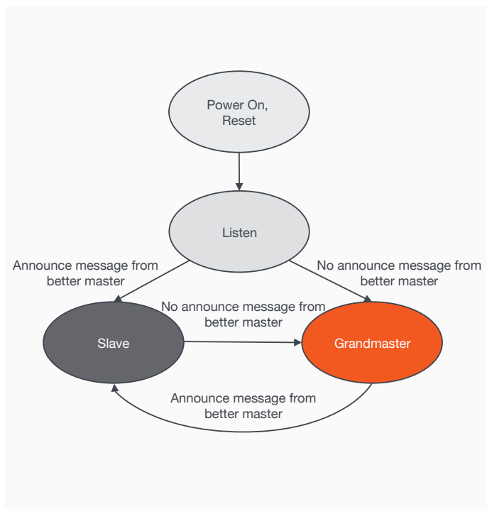
FIGURE 10. Determining Master/Slave Clock State.
