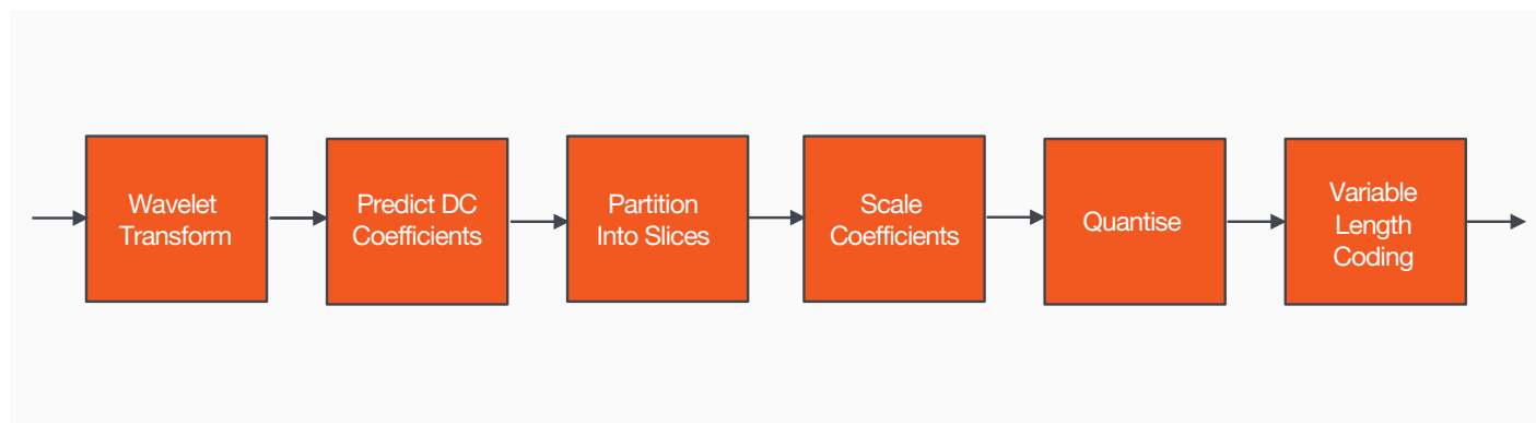
FIGURE 7. VC-2 Signal Processing Chain.
