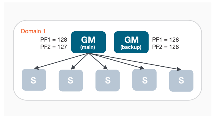
FIGURE 11. Configuration of Main/Backup Grandmasters for Automatic Failover.
