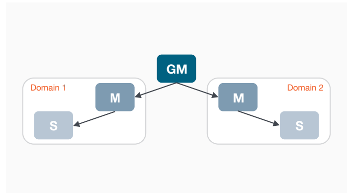
FIGURE 8. PTP Domains Synchronized to a Common Grandmaster.
