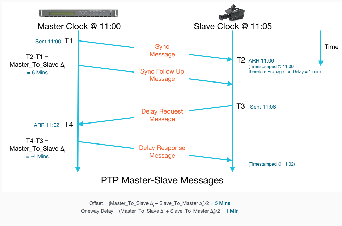
FIGURE 9. Deriving the Correct Time in a PTP Network.
