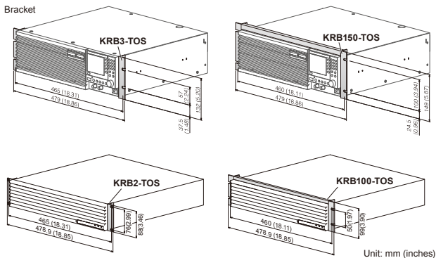
Bracket
