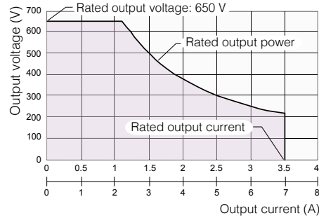
[PWX750HF/PWX1500H]
