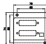
Dimensions wall mounting adapter
